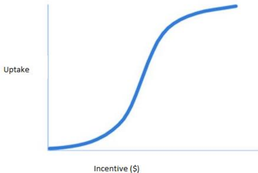
Figure 3: Uptake-Incentive Relationship 10
