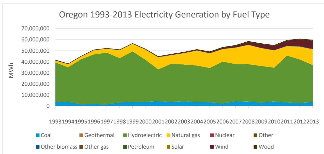
Figure 36: Oregon 1993-2013 Electricity Generation by Fuel Type 5
