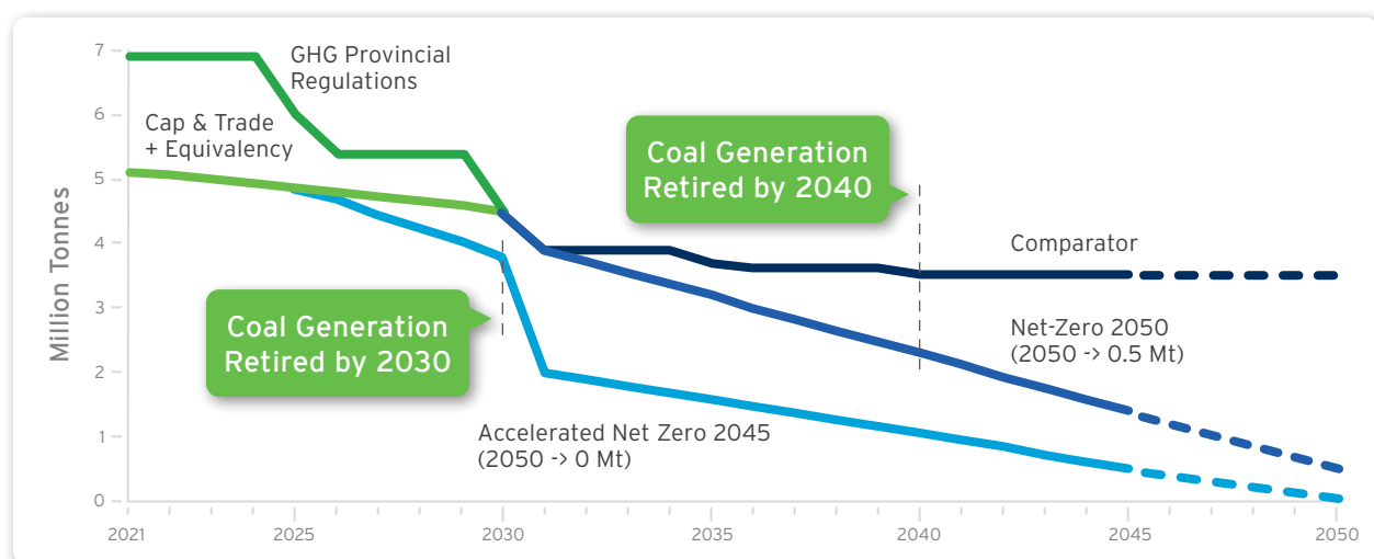
Figure 19. Greenhouse Gas Emissions Trajectories and Coal Retirements
