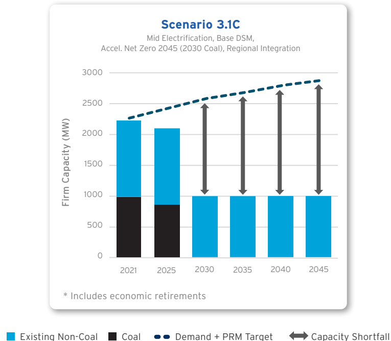
Figure 10. Existing Effective Capacity and Capacity Needs Under Scenario 3.1C
