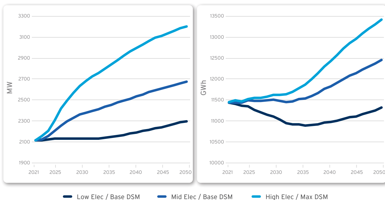
Figure 23. Firm Peak Load and Annual Energy Forecasts
