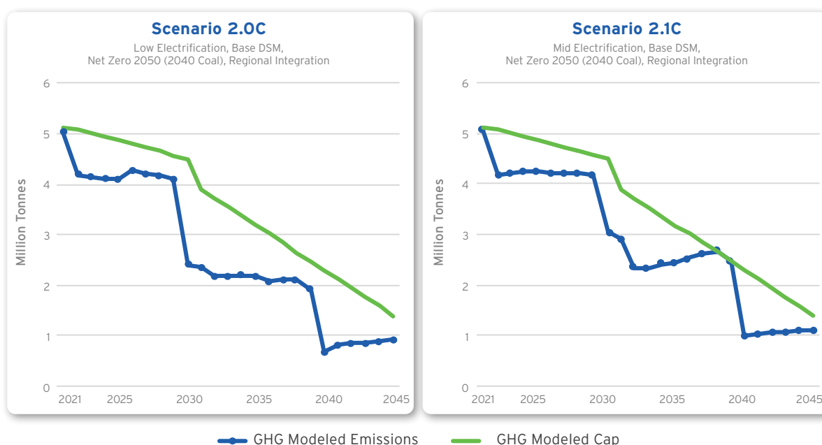
Figure 49. GHG Emissions in Scenarios 2.0C and 2.1C
