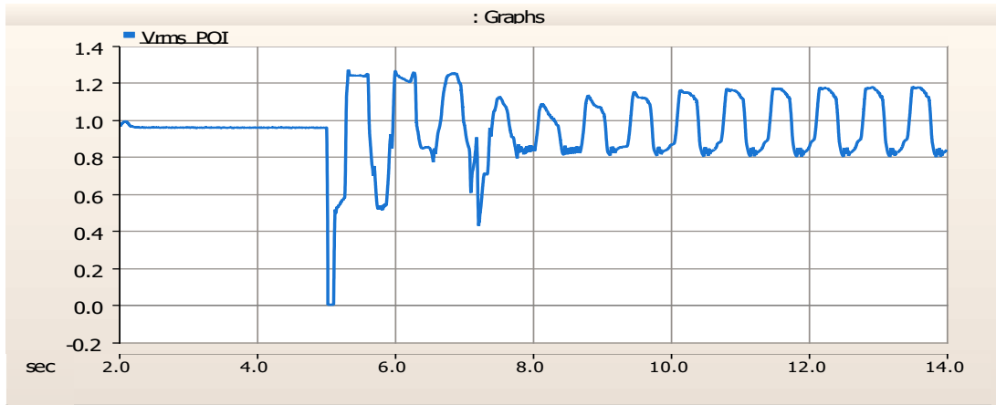
Figure 2: PSCAD™ Simulation Showing Unstable Oscillations
