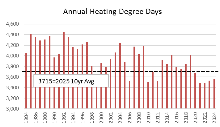
Figure 6: Historic Annual HDD
