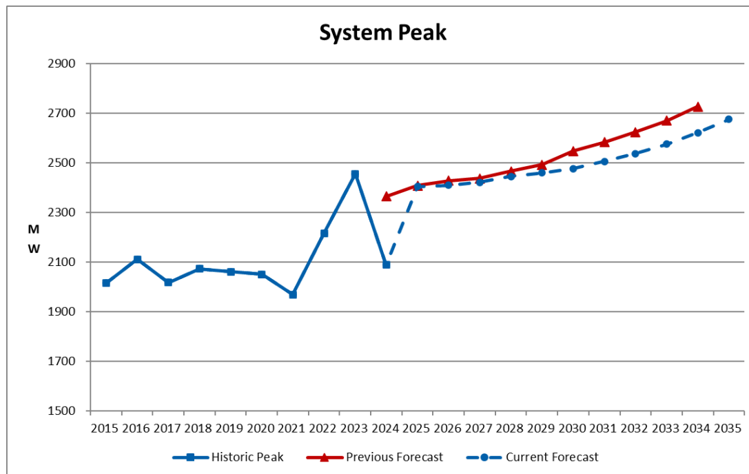
Figure 2: Historical and Predicted Annual System Peak
