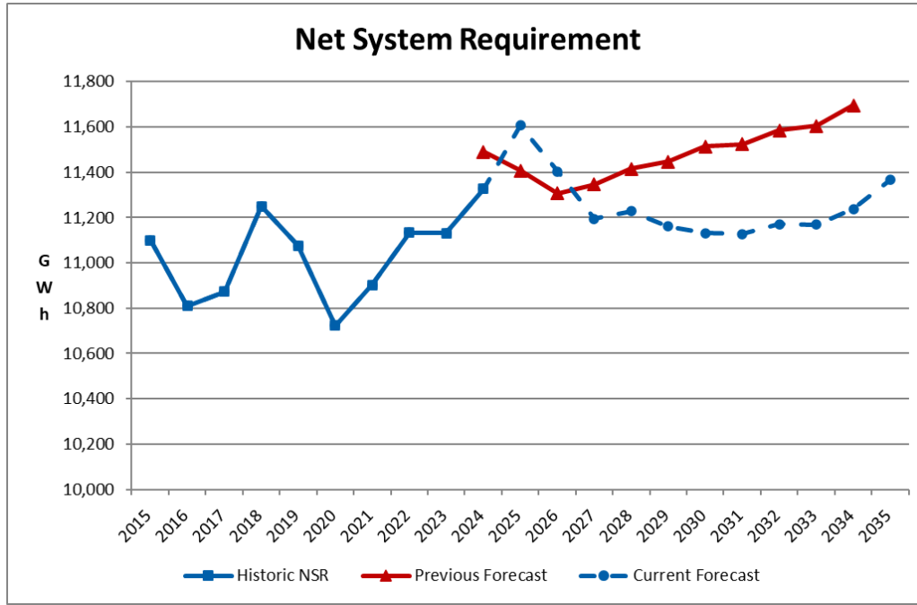
Figure 58: Historical and Forecast Annual NSR
