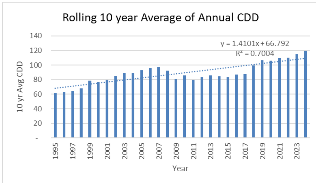
Figure 8: CDD Trend
