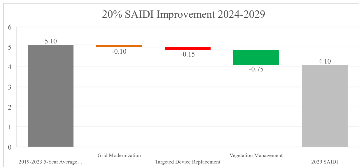
Figure 4: The Path to Improving SAIDI by 20 Percent
