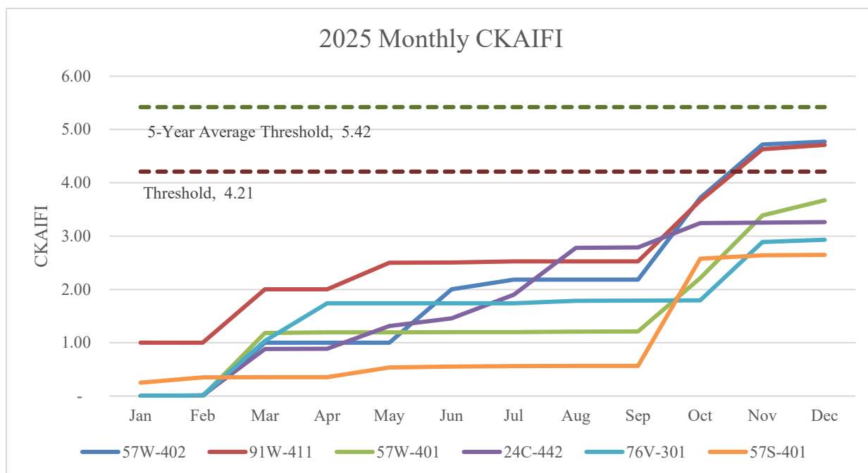
Figure 4 - 2025 Monthly CKAIFI
