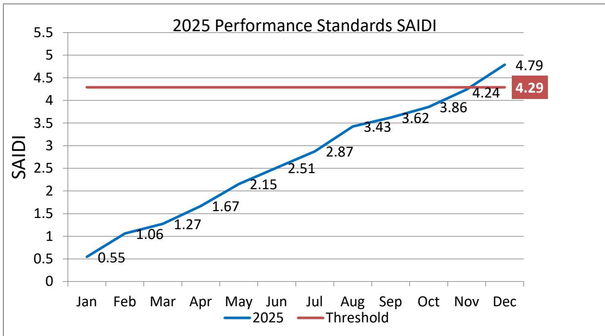
Figure 25 -2025 SAIDI Result
