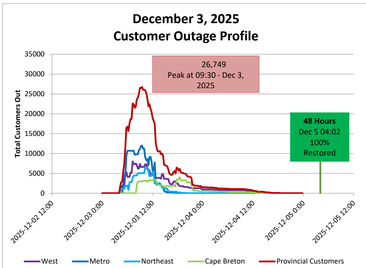
Figure 65 - December 3, 2025 Customer Outage Profile
