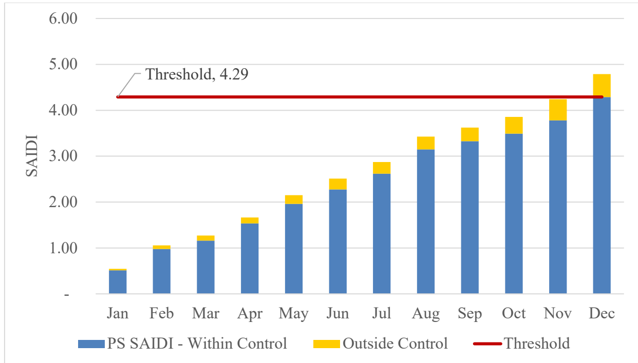
Figure 3 - 2025 Monthly SAIDI
