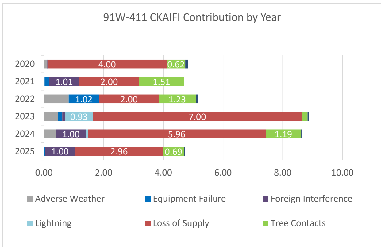
Figure 52 - 91W-411 CKAIFI Contribution by Year
