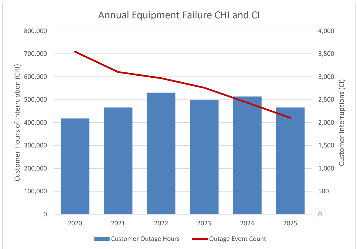
Figure 30 - Annual Equipment Failure Outage Hours
