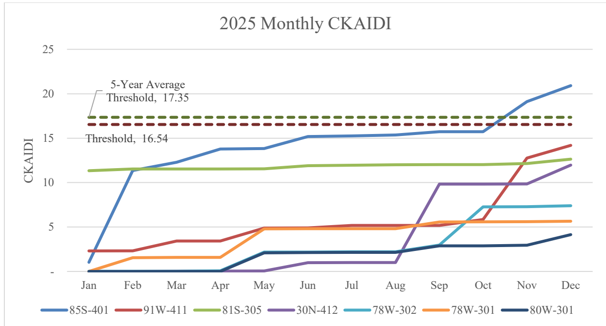
Figure 5 - 2025 Monthly CKAIDI
