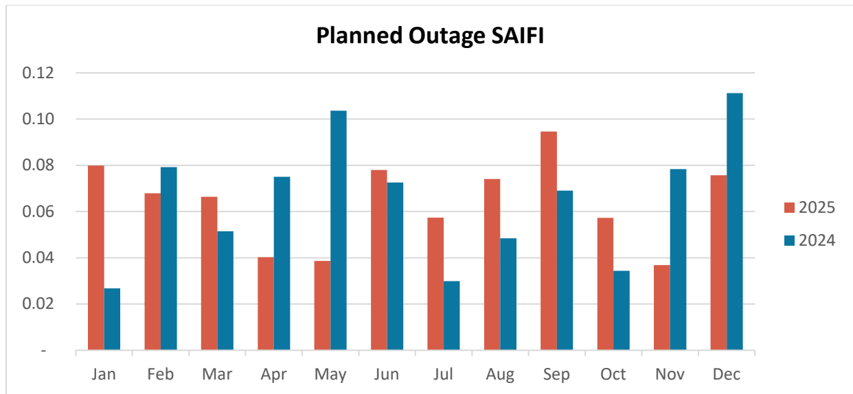
Figure 77 – 2024 and 2025 Planned Outage SAIFI by Month
