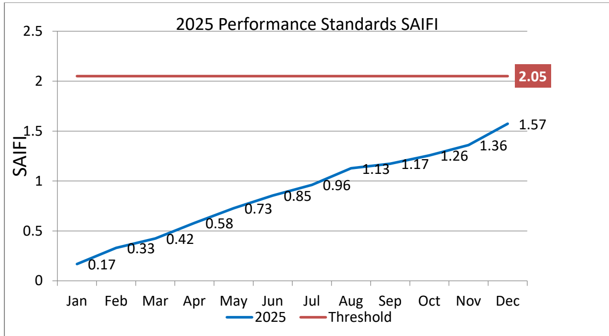
Figure 26 - 2025 SAIFI Result
