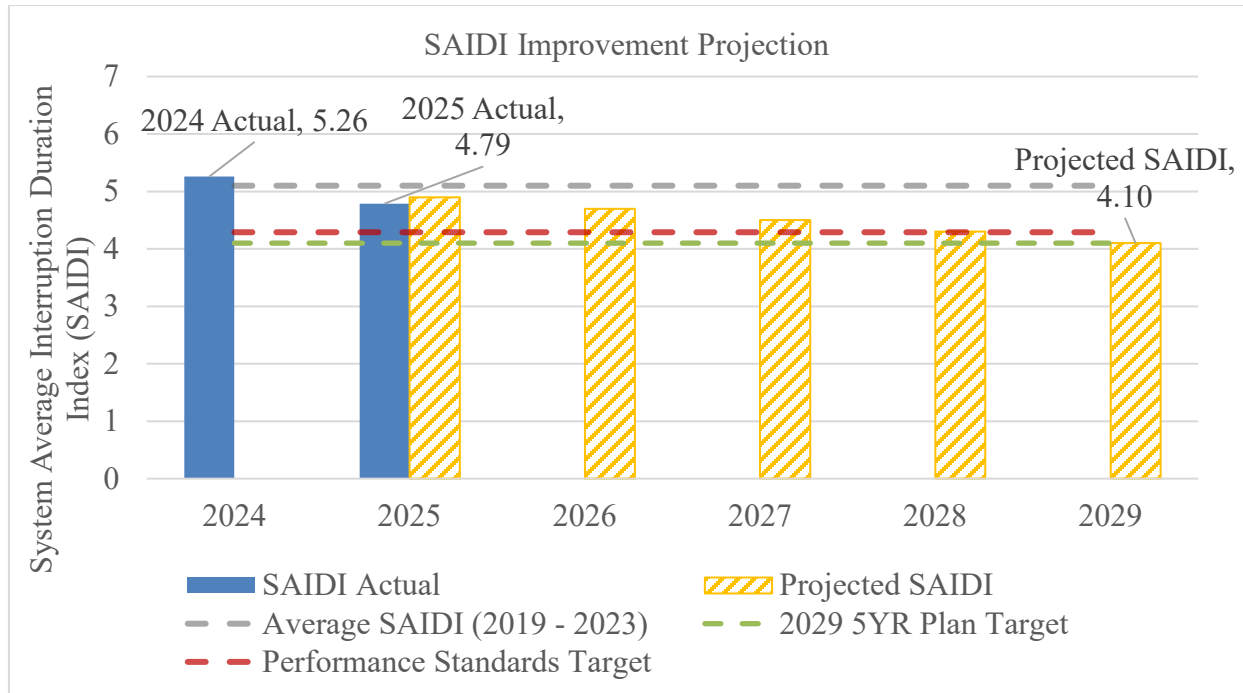
Figure 28 - SAIDI Improvement Projection
