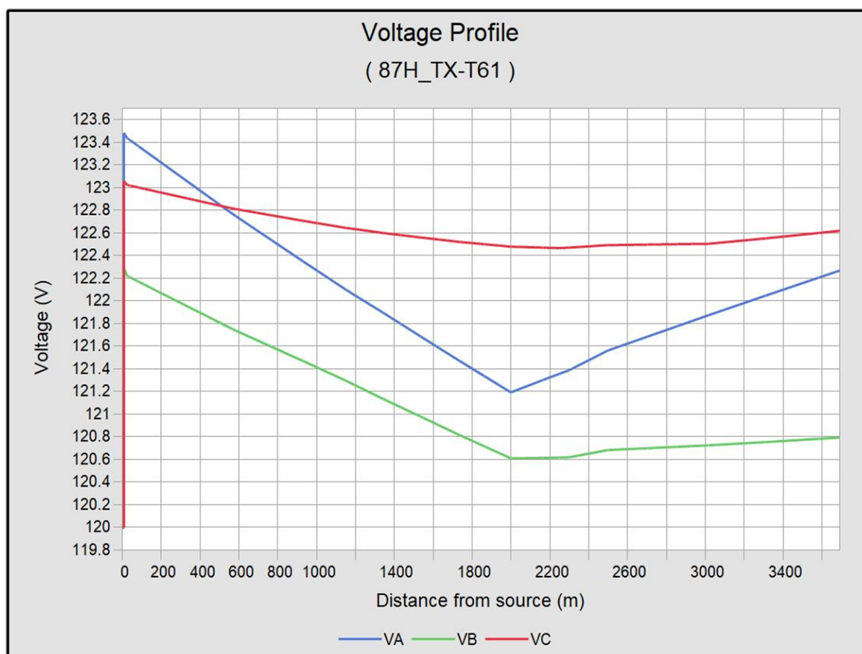
Figure 5: Voltage Profile at POI
