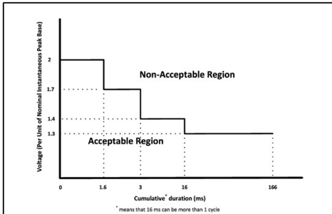
Figure 4: Transient Overvoltage Limits from IEEE 1547
